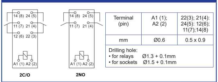
Connection Diagrams (pin side view)
