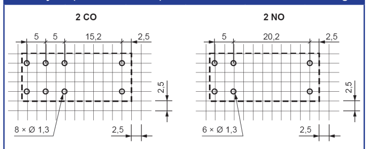
PCB Layout (solder side view)
