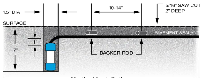
Vertical Installation
